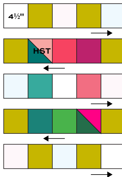
Block – Make 12
