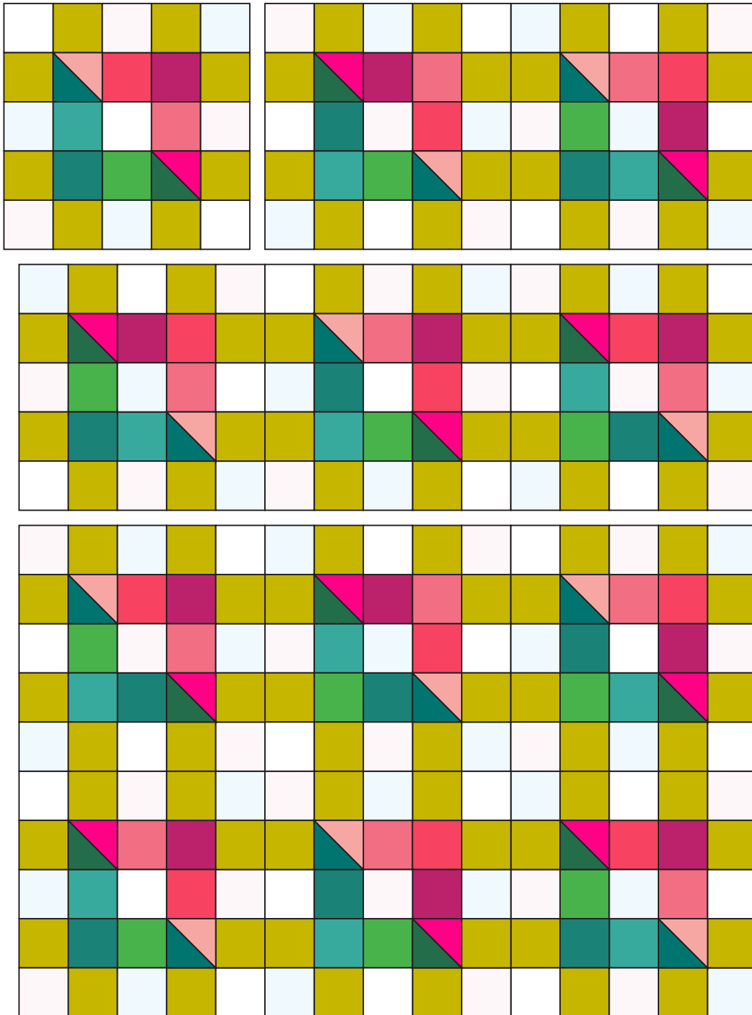
Quilt Diagram
