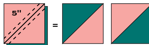
HST – Make 24
